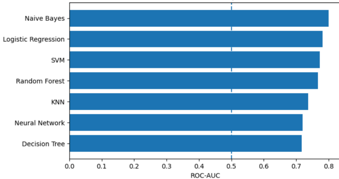
Model ROC-AUC Comparison
